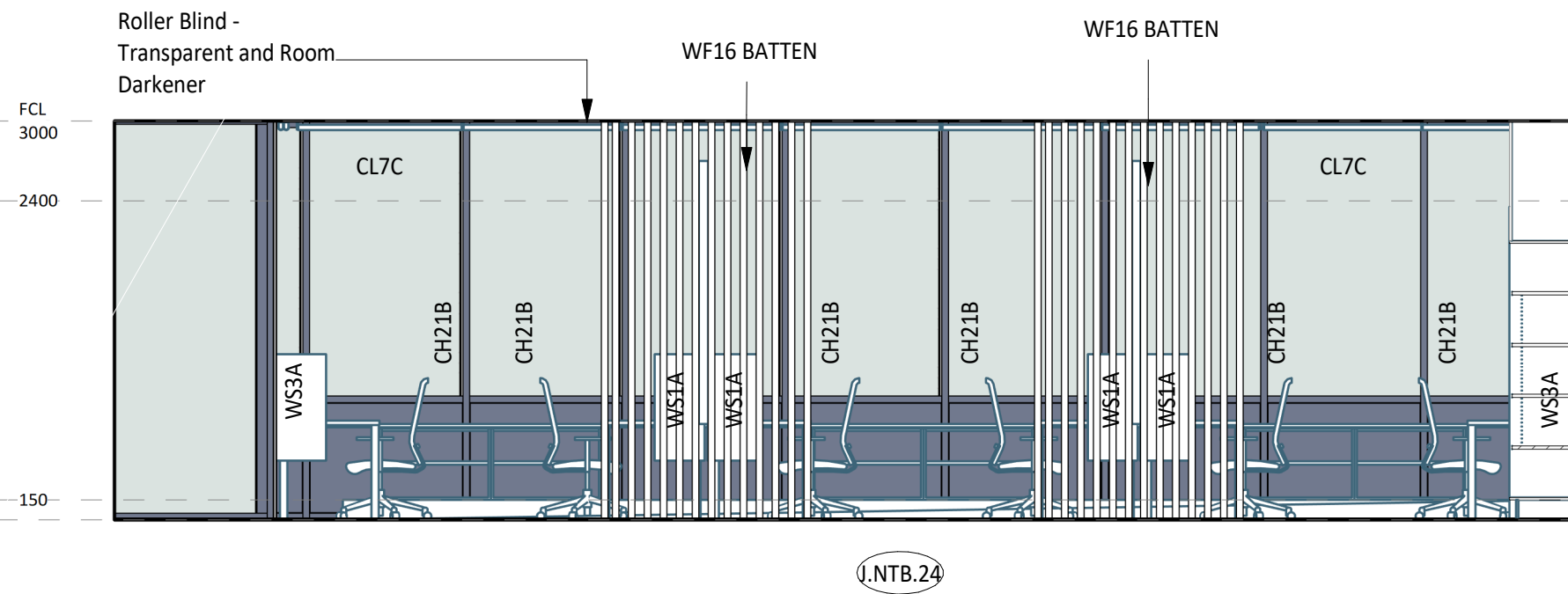
3 ELEVATION DETAIL 60-045 1 : 50
