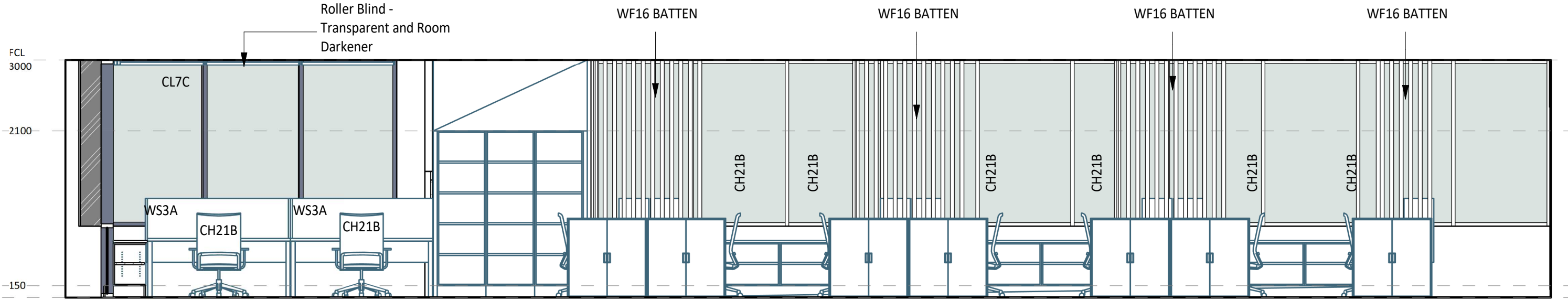
2 ELEVATION DETAIL 60-045 1 : 50
