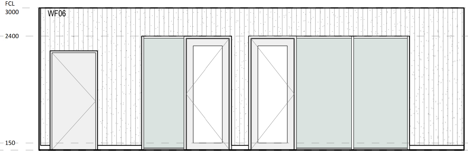
5 ELEVATION DETAIL 60-045 1 : 50
