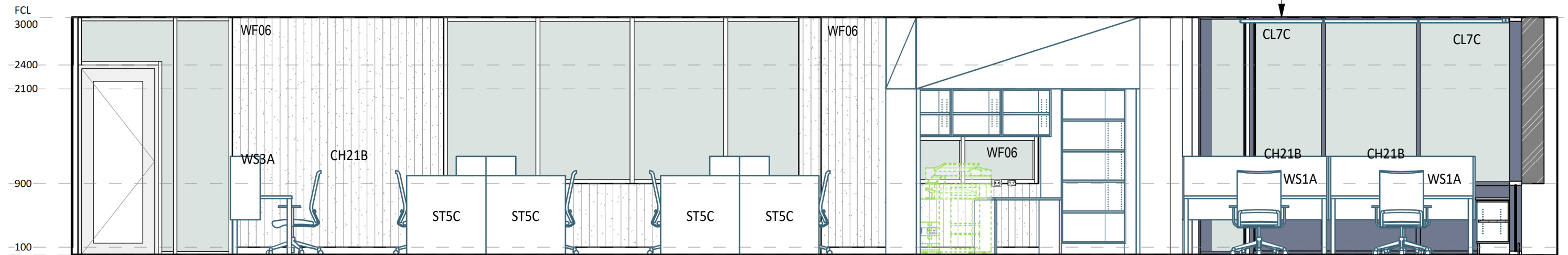
2 ELEVATION DETAIL 60-045 1 : 50
